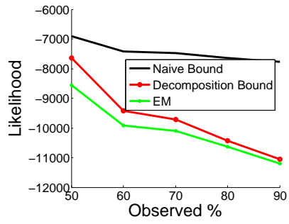
Figure 10: Upper bound for network Alarm.
