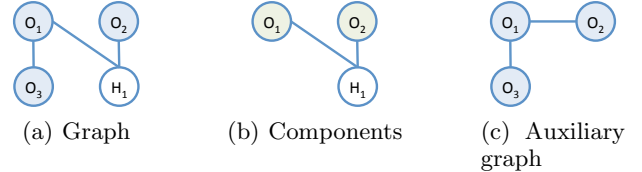
Figure 3: Auxiliary MRF graph under fully observed variables \mathbf{O} = \{O_1, O_2, O_3\} .
