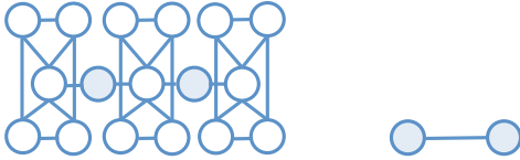
Figure 6: An MRF structure that leads to an auxiliary MRF of lower treewidth.
