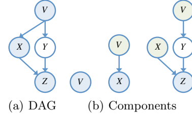
Figure 9: A DAG and its components under fully observed variables \mathbf{O} = \{V, X, Z\} .
