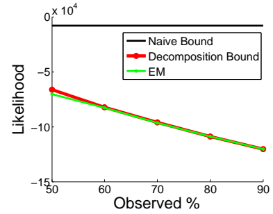
Figure 22: Upper bound for a tree network (255 nodes).
