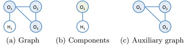
Figure 2: Auxiliary MRF graph under fully observed variables \mathbf{O} = \{O_1, O_2, O_3\} .
