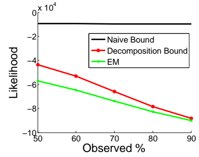
Figure 14: Upper bound for network Andes.
