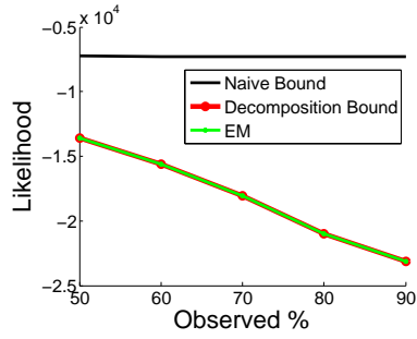
Figure 18: Upper bound for a chain network (50 nodes).
