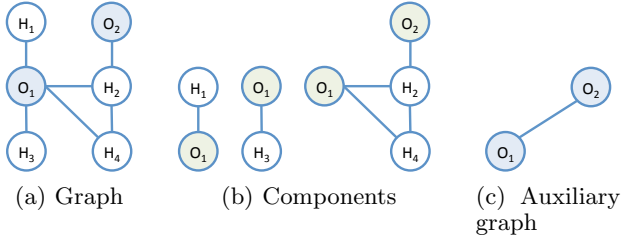
Figure 1: Auxiliary MRF graph under fully observed variables \mathbf{O} = \{O_1, O_2\} .
